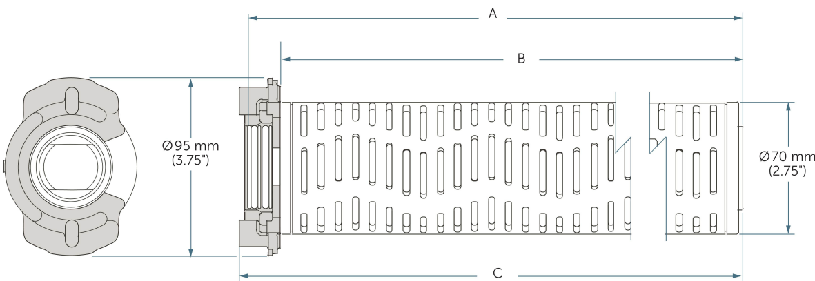
Code 0 – End View with Chemlock Key on Cartridge
